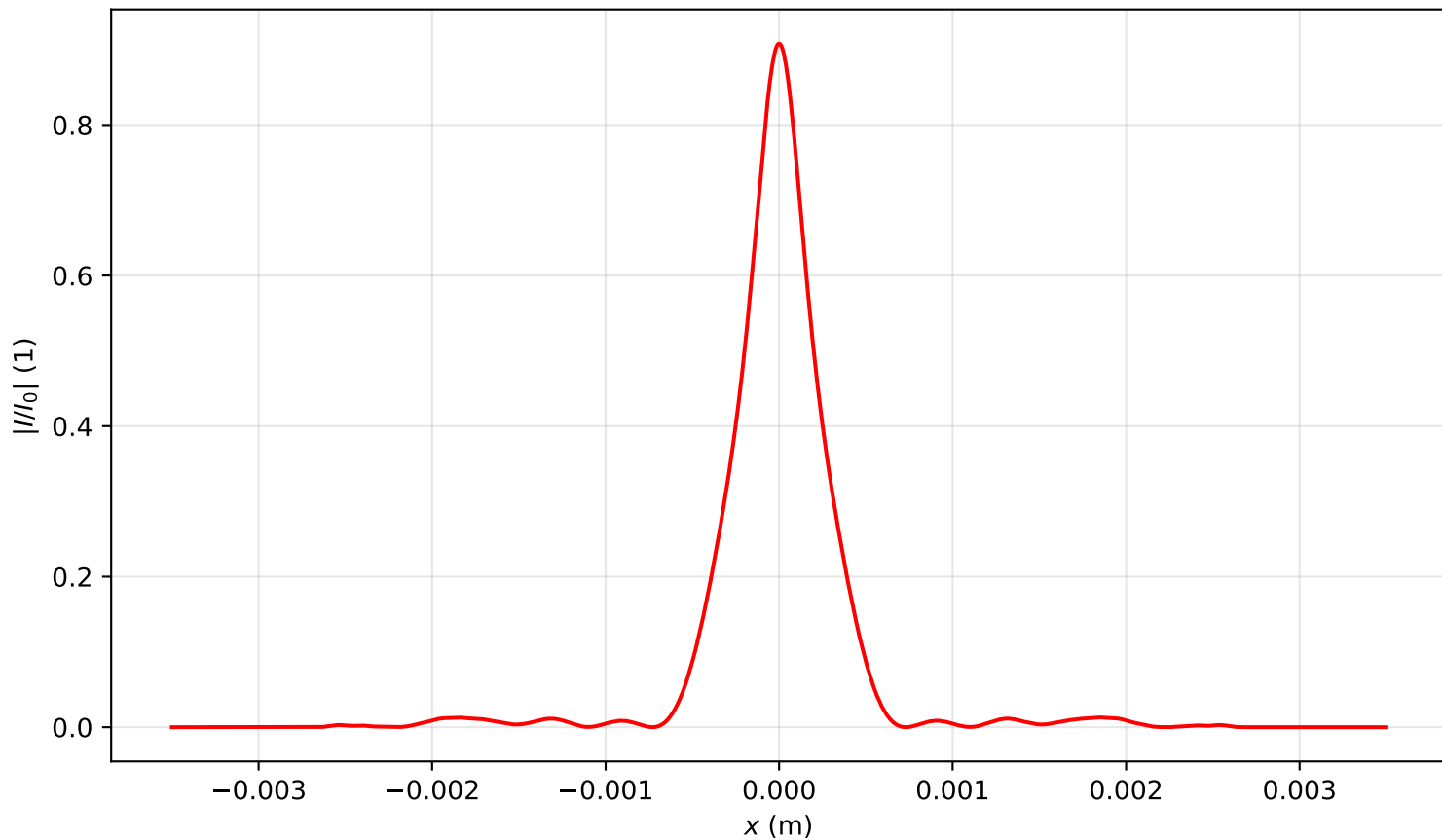
Intensity profile I(x, y = 0, z = 0.796)/I_0 , P_{in}=4.0P_{cr} , artificial time
